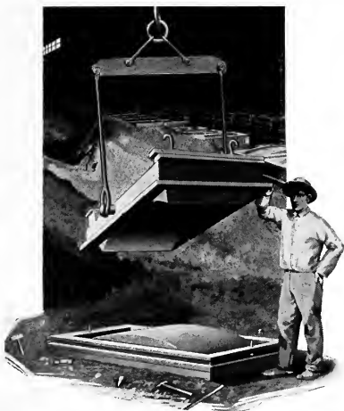
Fig. 12. Tunnel Segment Mould—Upper half or Cope—Made on a 42" x 97" plain jolt-moulding machine.
